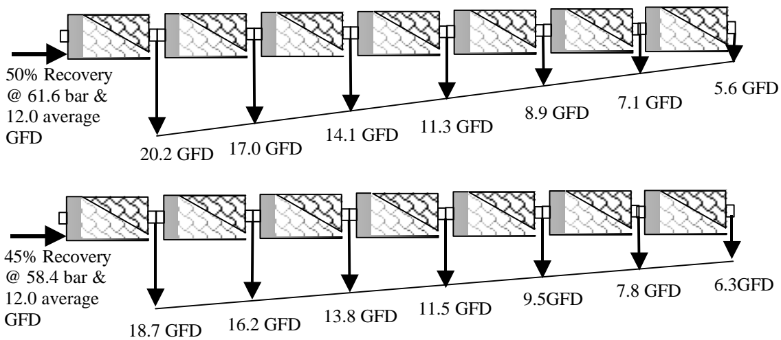
Figure 4. Element By Element Flux at Various Conversion Rates
