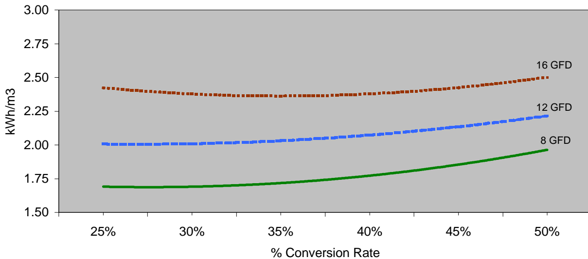
Figure 3. SWRO PX kWh/m 3 Vs Conversion Rate @ various GFD's (2)
