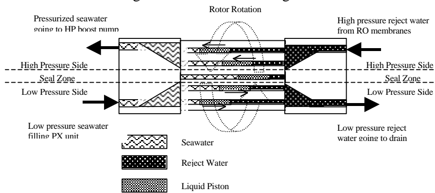
Figure 1. Pressure Exchanger Flow Path
