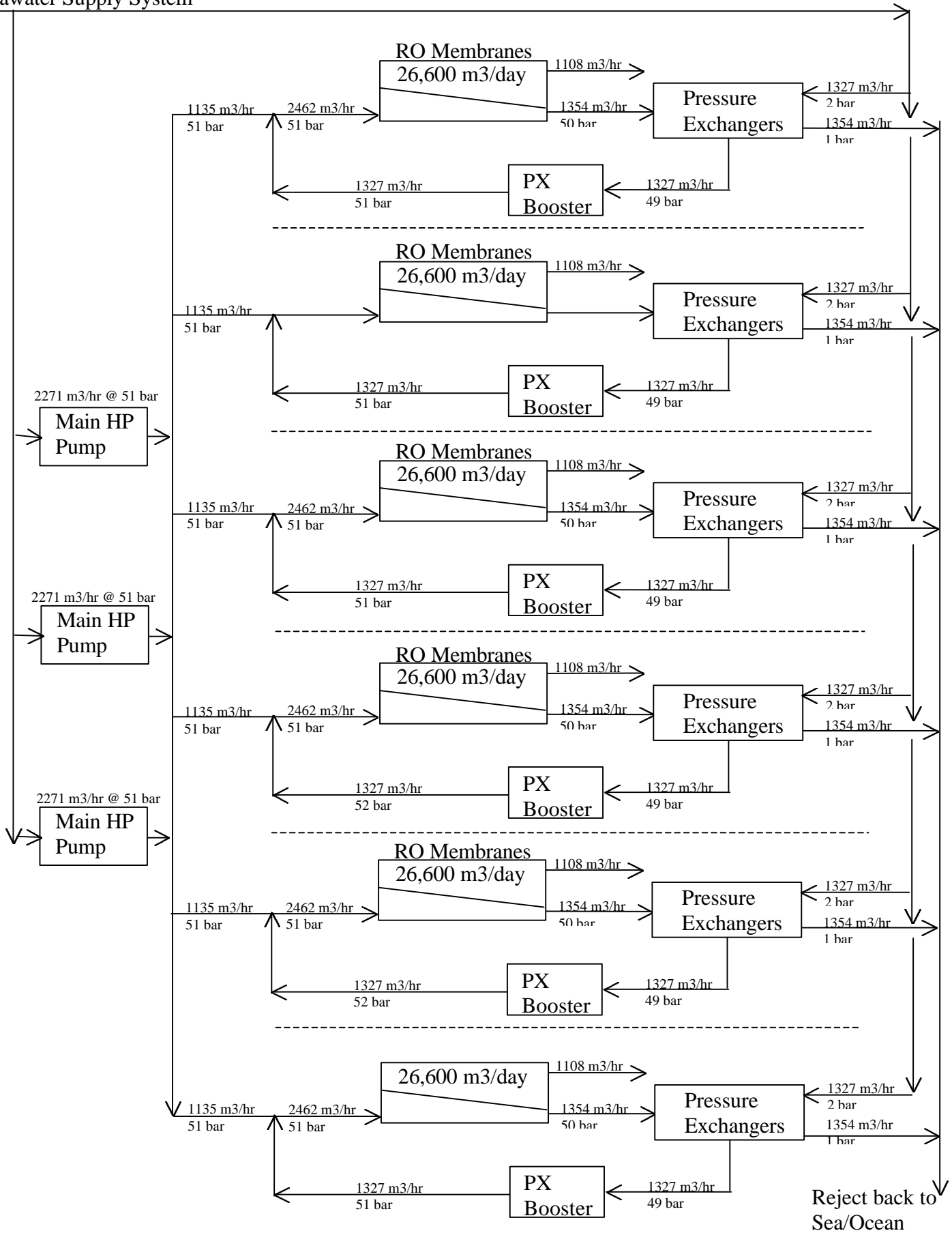
Figure 6. 159,600 m 3 /day System in 6ea 26,600 m 3 /day Trains.
