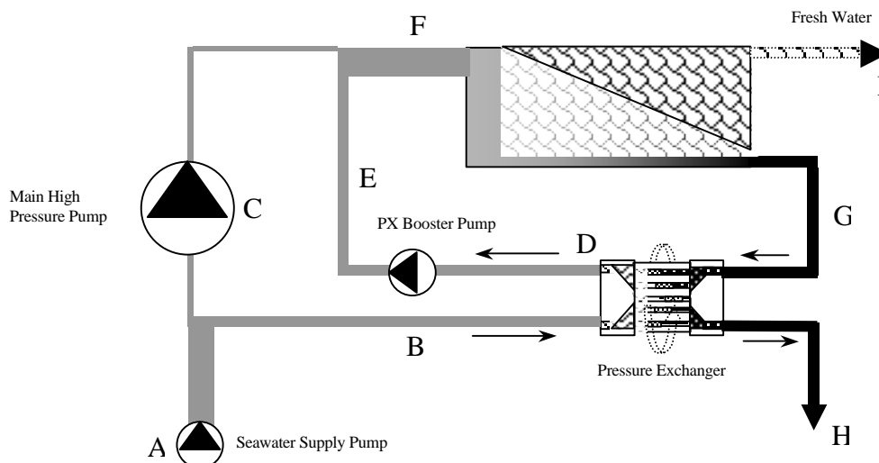
Figure 2. Typical System Flow Path
